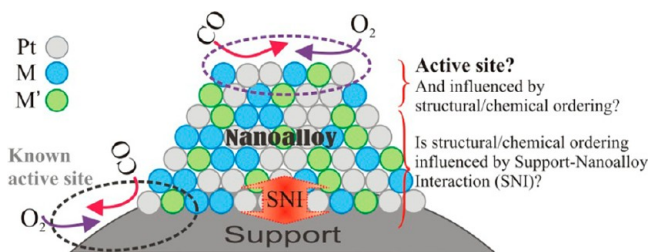
Scheme 1. A Schematic Illustration of the Oxidation Reaction of Carbon Monoxide with Oxygen as a Probe Reaction to the Active Sites on a Supported Nanoalloy Catalyst
