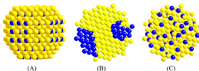
Figure 7. Chemical order–disorder effects in supported \text{Pt}_{39}\text{Ni}_{22}\text{Co}_{39} nanoparticles: chemically ordered structure for the carbon-supported particles prepared by the nonoxidative–reductive treatment (A), phase segregated structure on the silica-supported particles (B), and chemically disordered (random alloy) structure for the titania-supported particles and the carbon-supported particles prepared by the oxidative–reductive treatment (C). Transition base metals are in yellow, Pt is in blue. The configurations feature cubic type ordering where the relative concentration of transition base metal atoms (Co/Ni) to Pt atoms is 3:1. The chemically ordered model is based on the archetypal (noble metal)(transition metal) 3 (e.g., \text{AuCu}_3 -type) structure.
