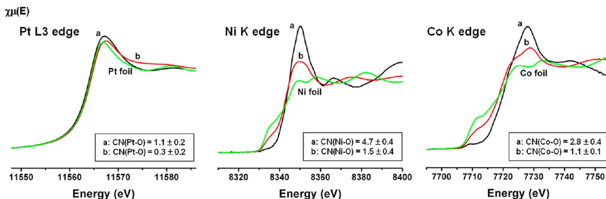
Figure 10. XANES spectra at Pt L3 edge, Ni K edge and Co K edge for Pt 39 Ni 22 Co 39 /C catalysts treated at (a) 260 °C in 15 vol % O 2 (oxidative atmosphere) only and (b) 15 vol % O 2 (oxidative atmosphere) followed by treatment at 400 °C in 15 vol % H 2 (reductive atmosphere).
