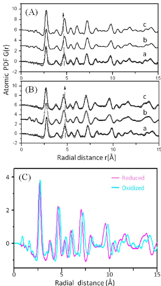
Figure 8. Atomic PDFs for Pt 25 Ni 16 Co 39 nanoalloys supported on carbon obtained from in situ HE-XRD data collected under controlled temperature and oxidative (O 2 )/reductive (H 2 ) atmosphere. The catalyst was subjected sequentially to two different treatment conditions: (A) under 10 vol % O 2 (a) starting with room temperature (25 °C), (b) heating to 260 °C and (c) cooling back to room temperature; and (B) under 5 vol % H 2 (a) starting with room temperature, (b) heating to 400 °C, and (c) cooling back to room temperature. (C) Comparison of curves labeled c in panels A and B, revealing a significant difference in the positions of the PDF peaks, that is, of the interatomic distances in the samples subjected to different treatment.
