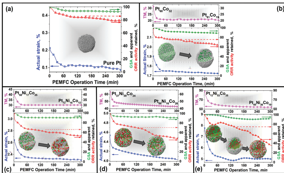
Fig. 6 Evolution of the atomic-level strain (blue symbols & line), GSA (green symbols & line), chemical composition (magenta symbols) and apparent ORR activity (red symbols & line) for pure Pt and Pt-TM nanoalloy catalysts deposited on the cathode of an operating PEMFC. Changes in the atomic-level strain are obtained from changes in the lattice parameter of the respective NPs as normalized against the lattice parameter of pure Pt. Changes in GSA values are obtained from changes in the FWHM of Bragg-like peaks in the respective in operando HE-XRD patterns as normalized against the GSA of fresh catalysts particles. Changes in the apparent electrocatalytic activity are derived from changes in the PEMFC “redox” current at 0.9 V on the respective polarization curves. MD-built & RMC refined 3D models as insets show the structural state of the fresh (model on the left) and active (model on the right) catalysts. The catalysts undergo the following evolution during the PEMFC operation: (a) fresh Pt NPs relax a bit and retain their fcc-type structure; (b) {chemically ordered} \text{Pt}_{68}\text{Co}_{32} NPs transform into {chemically disordered} NPs whose surface is depleted of Co atoms; (c) {near random alloy} \text{Pt}_{58}\text{Ni}_{17}\text{Co}_{25} NPs transform into {largely Pt NPs comprising small domains of TM atoms}; (d) {near random alloy} \text{Pt}_{37}\text{Ni}_{39}\text{Co}_{24} NPs transform into {TM rich core-Pt rich shell} NPs; and (e) {fully TM core-patchy Pt skin} \text{Pt}_{12}\text{Ni}_{53}\text{Co}_{35} NPs transform into an intermediate active state with a {fully TM core-thick Pt shell type} structure. This state evolves with further cycling and becomes of a {TM rich core-Pt rich shell} type. This is to be expected given both the specific structure of the fresh NPs and extensive change in their chemical composition with cycling. Note that the observed changes in the chemical composition, local strain, overall atomic arrangement and apparent ORR activity are highly correlated in terms of onset, duration and magnitude, indicating the presence of an instant link between these fundamental characteristics of nanoalloy catalysts. A more detailed rendition of the structure models is given in Fig. S12.† Pt, Co and Ni atoms are in grey, green and red, respectively.
