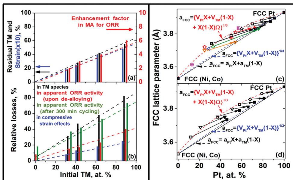
Fig. 7 (a) Residual TM percentage (black bars) and atomic-level strain (blue bars) in partially de-alloyed Pt-TM NPs. Enhancement (red bars) in the electrocatalytic activity (MA for ORR) of de-alloyed/activated NPs in comparison to pure Pt NPs obtained by complementary ex situ experiments. Dotted lines emphasize the correlation between the composition, structure and catalytic activity of the NPs. (b) Relative losses in TM species (black bars) and apparent ORR activity (initial loss/red bars and total loss/green bars) experienced by fresh Pt-TM alloy NPs inside the operating PEMFC. Changes in the local atomic strain (blue bars) are also shown. Comparison between the respective data sets in (a) and (b) indicate that, regardless having suffered large loss in activity in comparison to their pristine state, partially de-alloyed Pt-TM NPs perform better as ORR catalysts in comparison to pure Pt NPs. (c) Literature data for the fcc-lattice parameters of purposefully de-alloyed (closed symbols) and respective fresh (open symbols) Pt-TM alloy NPs (TM = Ni, Co and/or Cu). Data in black are for 4 nm Pt–Ni particles synthesized at 160 °C to 240 °C. 17 Data in gray are for commercial (E-Tek) 5.4 nm Pt–Co particles. 18 Data in green are for 20 nm polyhedral Pt–Ni particles. 19 Data in orange are for 5 nm Pt–Cu particles annealed at 950 °C. 6 Magenta rectangle denotes data for 3 nm wide and 100 nm long Pt 59 Ni 49 nanowires annealed at 260 °C. 92 Red star denotes data for sub-nanometer PtNiCo nanowires synthesized at 160 °C. 20 Red cross denotes data for space-confined 3 nm Pt–Ni particles annealed at 850 °C. 21 Red pentagon denotes data for 3 nm Pt–Co particles annealed at 950 °C. 22 Crossed magenta circle denotes data for 12 nm Pt–Ni particles annealed at 400 °C. 23 Crossed blue square denotes data for sputtered Pt–Ni nanoalloys. 28 Red stars denotes data for 9 nm Pt–Ni octahedra synthesized at 230 °C. 24 (d) FCC-lattice parameters for 300 min cycled (closed symbols) and respective fresh (open symbols) Pt-TM alloy NPs obtained by in operando experiments. Circles denote Pt 79 Ni 21 NPs discussed in ref. 87. Rhombuses denote data for Pt 68 Co 32 NPs. Squares denote data for Pt 58 Ni 17 Co 25 , Pt 37 Ni 39 Co 24 and Pt 12 Ni 53 Co 35 NPs. Triangles denote data for Pt 51 Co 18 Cu 31 and Pt 21 Ni 40 Cu 39 NPs. In (c) and (d) blue dotted lines represent the expected composition dependence of the lattice parameter for Pt-TM random alloys obtained from the elemental volumes of Pt and TM species (eqn (3)). Red dotted lines represent the expected composition dependence of the lattice parameter for Pt-TM alloy obtained from the elemental volumes of the intermixed atomic species plus a quadratic correction term involving a quantity \Omega referred to as an “excess volume” in the text (eqn (4)). Slanted black lines represent the composition dependence of the lattice parameter for Pt-TM random alloys as predicted by Vegard’s law (eqn (2)). Solid arrows link data for a given pair of cycled and respective fresh catalysts.
