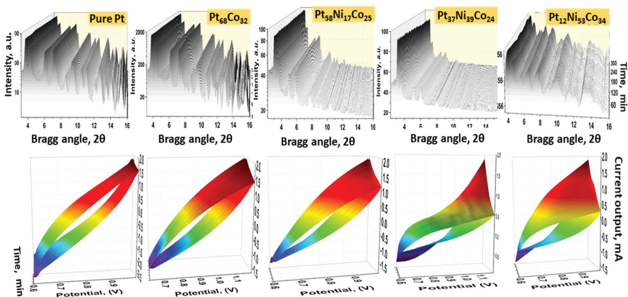
Fig. 1 (top row) Experimental in operando HE-XRD patterns ( \sim 300 in number) for pure Pt and Pt-TM alloy NPs (TM = Ni, Co) cycled inside the PEMFC for about 5 hours. (bottom row) Also shown are the concurrently collected polarization curves ( \sim 1600 in number) representing the PEMFC current output resulted from the repetitive application of external voltage in the range from 0.6 V to 1.0 V at a rate of 50 \text{ mV s}^{-1} . The curves tend to collapse with the potential cycling indicating a deterioration in the apparent ORR activity of the NPs for reasons discussed in the text. As shown in Fig. S5, † the magnitude and rate of the collapse with the potential cycling is significant and different for the different NPs. Selected polarization curves are shown in Fig. S3. †
