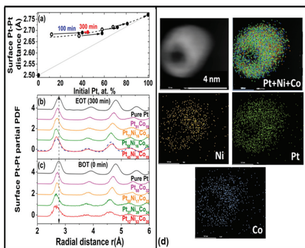
Fig. 8 (a) Average surface Pt–Pt distance in fresh (open circle) and 300 min cycled (solid circle) pure Pt and Pt–TM alloy NPs. The distance is obtained from the position of the first peak in the surface Pt–Pt partial PDFs for fresh (beginning of test/BOT) and 300 min cycled (end of test/EOT) NPs computed from the respective 3D models shown in Fig. 6. The PDFs are shown in (c) and (b), respectively. Broken line in (a) is a guide to the eye. Solid slanted line in (a) connects the bulk values for TM–TM and Pt–Pt bonding distances. Vertical broken lines in (b) and (c) mark bulk Pt–Pt bonding distance. (d) Representative HAADF–STEM image and elemental maps of a \text{Pt}_{45}\text{Ni}_{33}\text{Co}_{22} nanoparticle cycled for 600 min 87 . Due to the prolonged cycling and leaching of TM species, the nanoparticle has become near hollow. Nevertheless, its shell has remained a Pt–TM nanoalloy.
