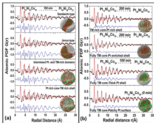
Fig. 5 (a) In operando (symbols) and computed (red line) atomic PDFs for \text{Pt}_{12}\text{Ni}_{53}\text{Co}_{35} alloy NPs cycled for 100 min. The computed PDFs are derived from structure models shown as insets. Residual difference (blue line) between the experimental and model computed PDFs is shifted by a constant factor for clarity. The difference is large, indicating the inability of the models to reproduce the experimental data. (b) In operando (symbols) and computed (red line) atomic PDFs for \text{Pt}_{12}\text{Ni}_{53}\text{Co}_{35} alloy NPs cycled for 0, 100, 200 and 300 min. The computed PDFs are derived from structure models shown as insets. Residual difference (blue line) between the experimental and computed PDF data is small, indicating the high quality of the respective models. A more detailed rendition of models in (a) and (b) is given in Fig. S11.† Pt, Co and Ni atoms are in gray, green and red, respectively. Note that, due to leaching of TM species during the potential cycling, the chemical composition of cycled NPs changes as shown in the plots (follow the horizontal broken lines).
