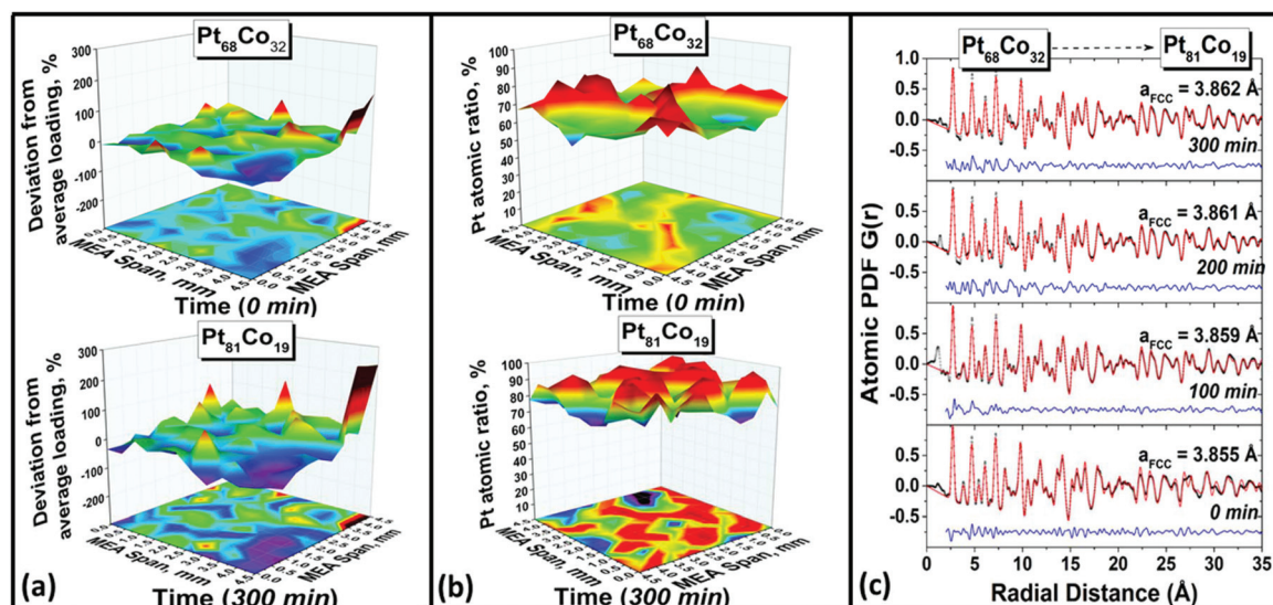
Fig. 3 (a) Mass distribution (loading) of fresh (top row) and 300 min cycled (bottom row) \text{Pt}_{68}\text{Co}_{32} alloy NPs particles over a 4.5 mm \times 4.5 mm area of the MEA. The distribution is irregular showing large fluctuations (up to \sim 100\% ) from the average catalyst loading for that area. (b) Distribution of Pt species over the same MEA area for fresh (top row) and cycled (bottom row) NPs. The distribution is normalized against the average chemical composition of the NPs, as determined by EDS. Note that, due to leaching of Co species during the PEMFC operation, the average chemical compositions of the NPs changes from \text{Pt}_{68}\text{Co}_{32} to \text{Pt}_{81}\text{Co}_{19} . Nevertheless, the fluctuations of the chemical composition of the NPs at different spots of the MEA do not exceed a few at. %. (c) Experimental (symbols) and computed (red line) atomic PDFs for fresh and cycled \text{Pt}_{68}\text{Co}_{32} alloy NPs. The computed PDFs are derived from a structure model featuring a uniform fcc lattice. The duration of cycling and refined parameter of the model fcc-lattice are given for each data set. Residual difference (blue line) between the experimental and computed PDF data is shifted by a constant factor for clarity. Modeling quality factors R_w , defined in the ESI, † for all fits are in the order of 18 ( \pm 3 ) %.
