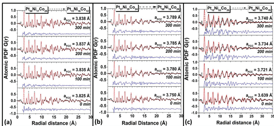
Fig. 4 Experimental (symbols) and computed (red line) atomic PDFs for fresh and cycled (a) \text{Pt}_{58}\text{Ni}_{17}\text{Co}_{25} , (b) \text{Pt}_{37}\text{Ni}_{39}\text{Co}_{24} and (c) \text{Pt}_{12}\text{Ni}_{53}\text{Co}_{35} alloy NPs. The computed PDFs are derived from a model featuring a uniform fcc-type lattice. The duration of cycling and refined parameter of the model fcc-lattice are given for each data set. Residual difference (blue line) between the experimental and computed PDF data is shifted by a constant factor for clarity. Modeling quality factors R_w , for fresh and cycled \text{Pt}_{58}\text{Ni}_{17}\text{Co}_{25} are in the order of 19 ( \pm 3 ) %. The modeling quality factor for fresh \text{Pt}_{37}\text{Ni}_{39}\text{Co}_{24} NPs is 20%. The modeling quality factor for 300 min cycled \text{Pt}_{37}\text{Ni}_{39}\text{Co}_{24} NPs deteriorates to 27%. Modeling quality factors for both fresh and cycled \text{Pt}_{12}\text{Ni}_{53}\text{Co}_{35} NPs are in the order of 30% to 40%, indicating that Pt and TM species in the NPs do not sit on the vertices of a uniform fcc-type lattice. Finite size models exhibiting non-uniform patterns describe the NPs to a much better extent (see Fig. 5b). Note that, due to leaching of TM species, the relative percentage of Pt in the cycled NPs increases during the PEMFC operation (follow the dotted arrows on top of the plots).
