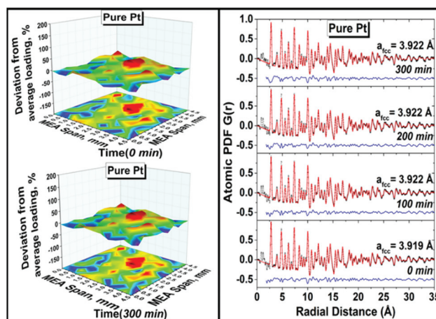
Fig. 2 (left) Mass distribution (loading) of fresh (top row) and 300 min cycled (bottom row) Pt NPs over a 4.5 mm \times 4.5 mm area of the MEA. The distribution does not exhibit large fluctuations about the average catalyst loading for that area. (right) Experimental (symbols) and computed (red line) atomic PDFs for fresh and cycled Pt NPs. The computed PDFs are derived from a model featuring a uniform fcc-type lattice. The duration of cycling and refined parameter of the model fcc-lattice are given for each data set. Residual difference (blue line) between the experimental and computed PDF data is shifted by a constant factor for clarity. Modeling quality factors, R_w , defined in the ESI,† for all fits are in the order of 15 ( \pm 3 ) %.
